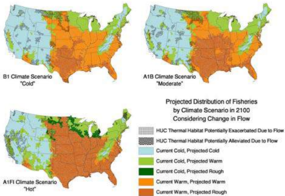
Figure 7.4. Projected change in distribution of coldwater, warmwater, and rough fish species in 2100 (source: Jones et al 2013).
